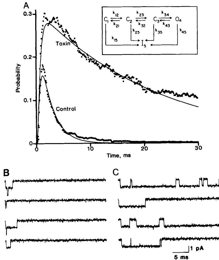
FIGURE 11. Model simulation of TsIV-5 effect on probability of single-channel opening ( A ) and single-channel bursting kinetics ( B and C ). Test potential -20 mV. In the kinetic model, rate constants that could be extracted directly from single-channel toxin data were constrained and the remaining rates were obtained by fitting the observed P_o to the model by an iterative curve-fitting procedure. In fitting the control P_o curve, all rate constants were constrained to equal those obtained in the toxin data, except k_{45} and k_{35} which were fit. The rate
